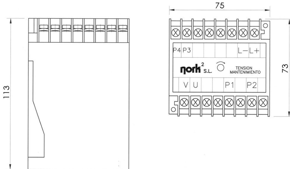
Overexcitation box.NS.01
